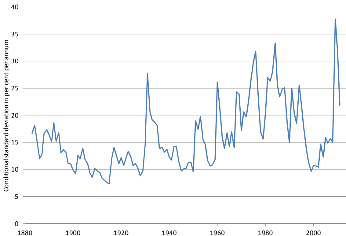
Figure 2.7 EGARCH estimates
